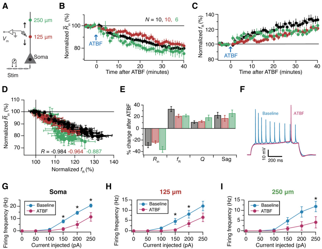
Figure 4. Antidromic Theta-Burst Firing Results in a Reduction in Excitability and an Increase in Resonance Frequency across the Somato-Apical Trunk
