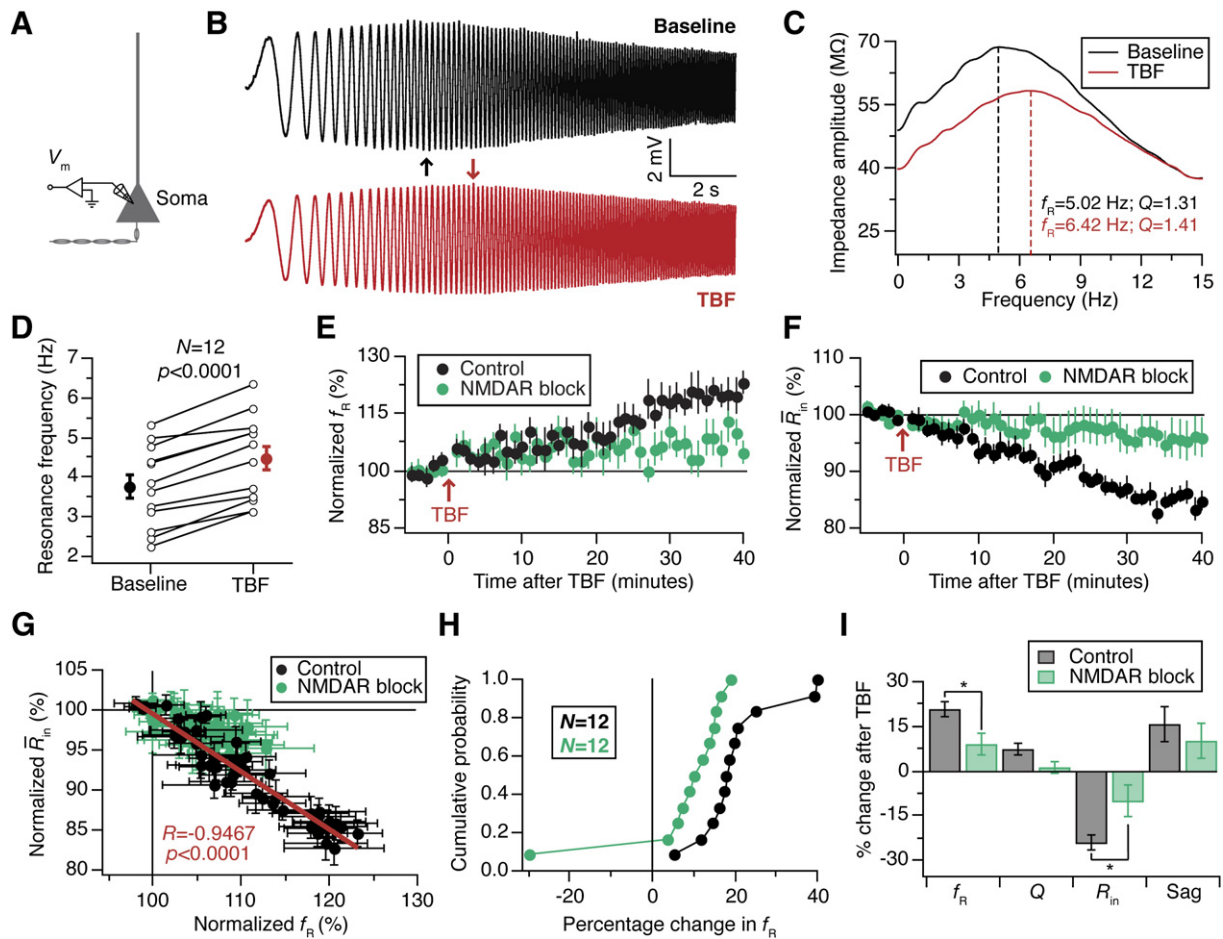
Figure 3. Theta-Burst Firing Elicits an NMDAR-Dependent Increase in Resonance Frequency
