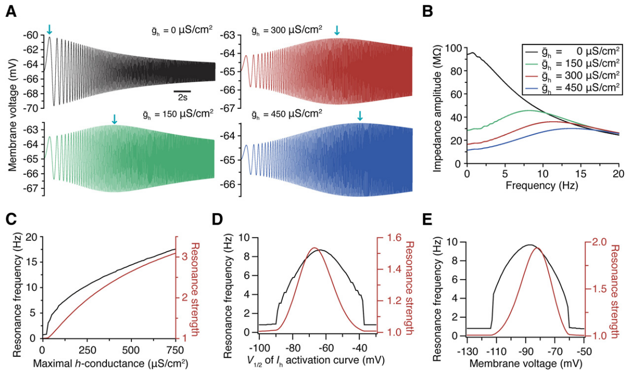
Figure 7. Simulations Reveal a Direct Relationship between Subthreshold Resonance and h -Channel Properties
