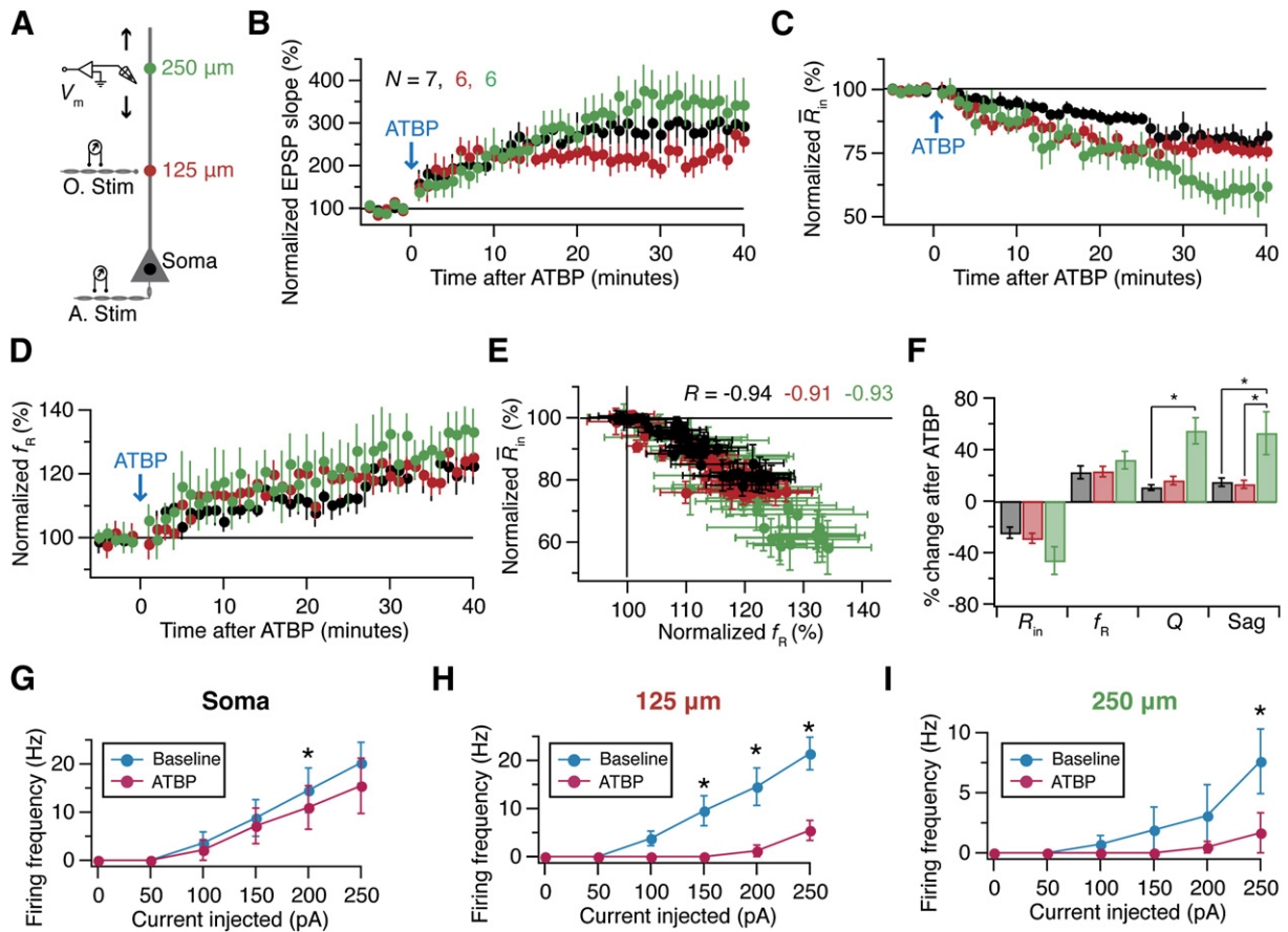
Figure 5. LTP Is Accompanied by a Reduction in Excitability and an Increase in Resonance Frequency across The Somato-Apical Trunk
