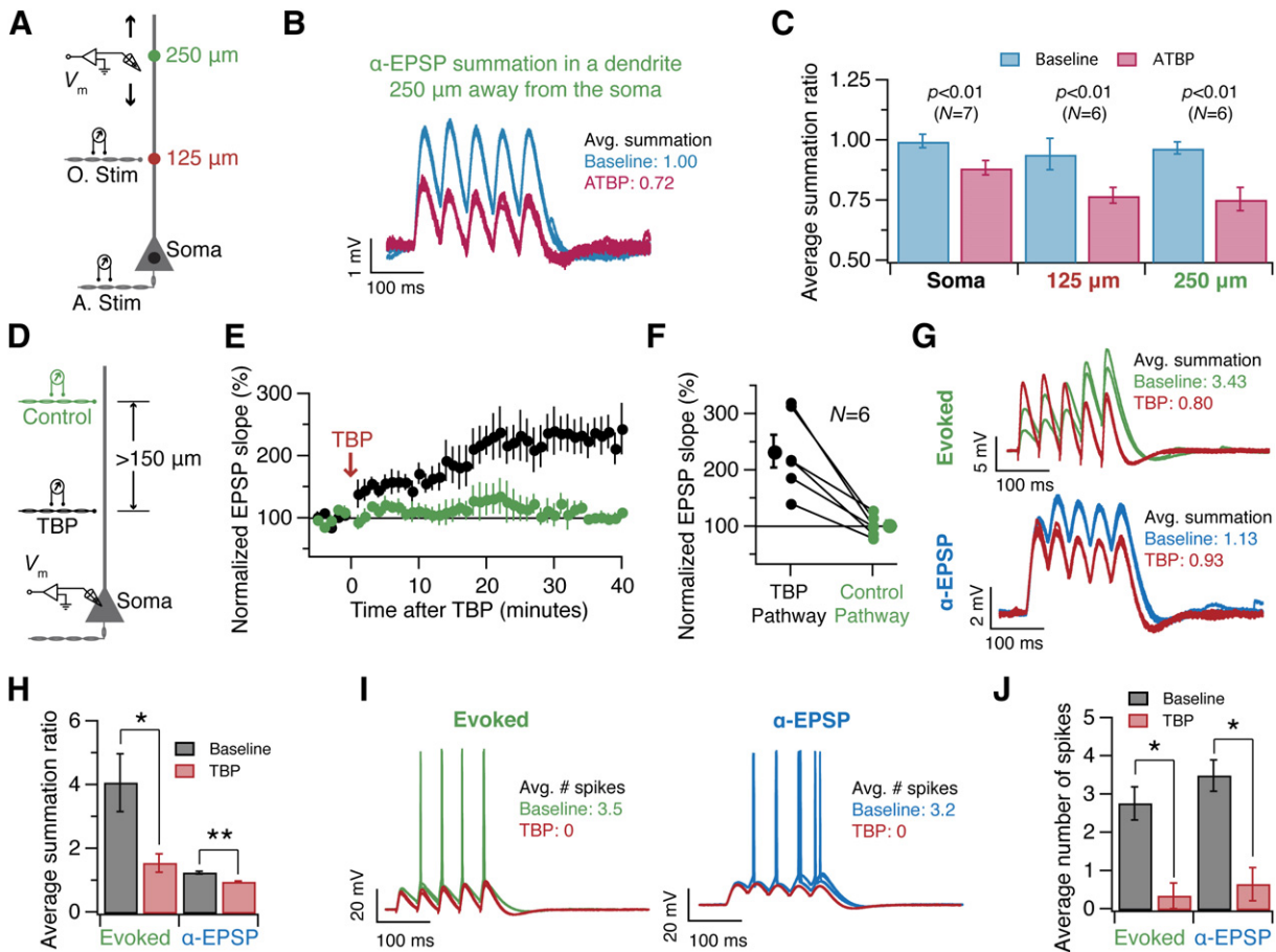
Figure 6. LTP Is Accompanied by a Nonlocal Reduction in Temporal Summation
