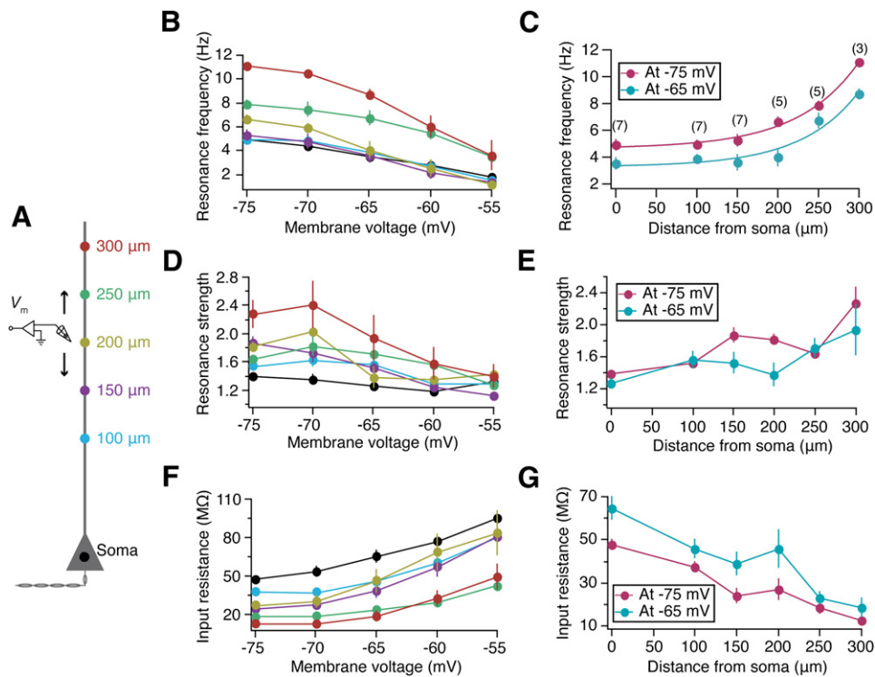
Figure 1. Resonance Frequency in Dendrites Increases Exponentially with Distance from the Soma
