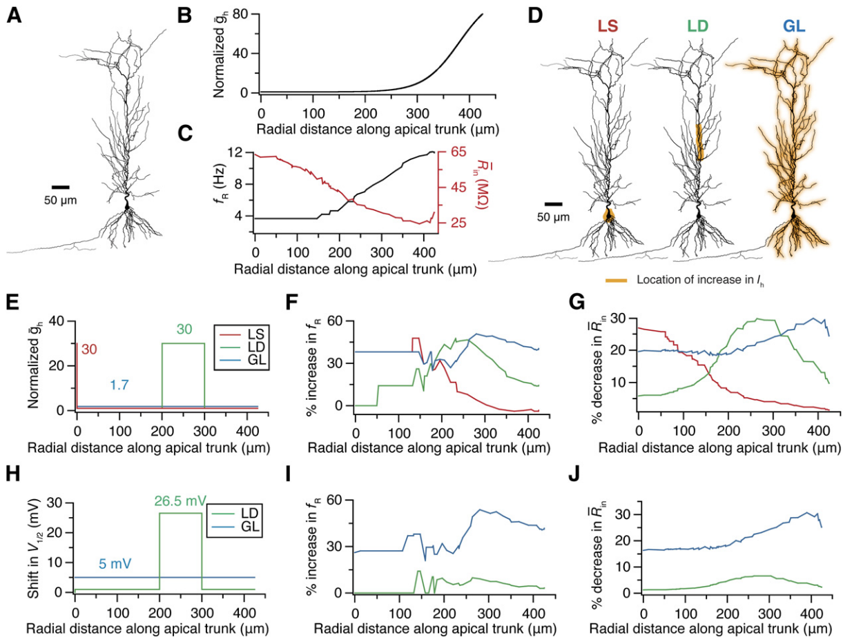
Figure 8. Multicompartmental Simulations Indicate that Plasticity in I_h Has to Express Globally to Elicit Global Changes in Resonance Frequency and Input Resistance
